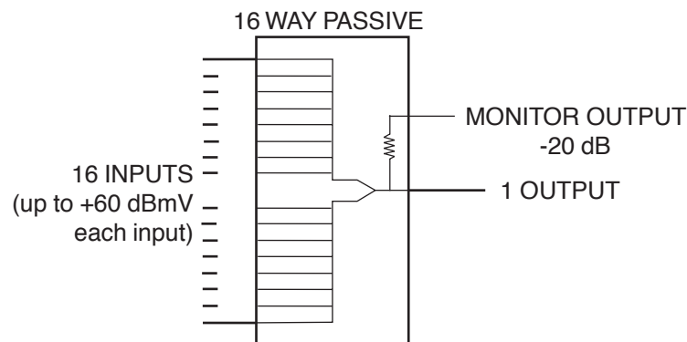
BLOCK DIAGRAM
